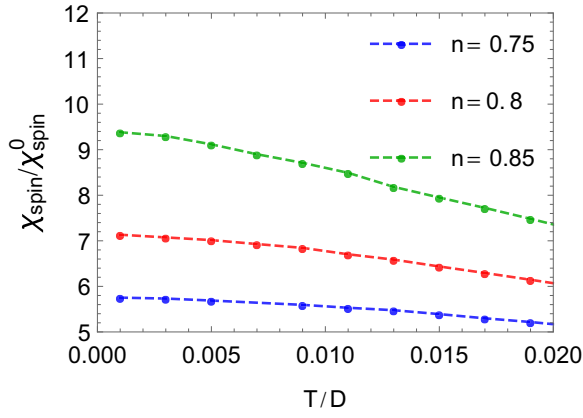
FIG. 14. Magnetic susceptibility (DMFT results). We note that the Stoner enhancement grows as \delta \rightarrow 0 and its T dependence is Pauli like but with a somewhat enhanced T dependence at higher n . The crossover to linear resistivity occurs (see Fig. 2) at fairly low T \lesssim .005D at these densities but has no reflection on the variation of \chi_{\text{spin}} . We may thus infer that spin disordering is not relevant to the linear resistivity seen here.
