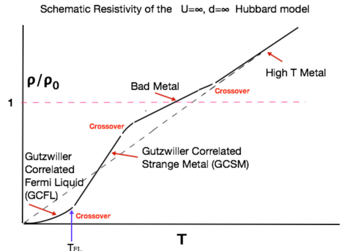
FIG. 1. A schematic view of the different regimes of temperature dependent resistivities found in the calculations of Refs. [5–8]. The various temperature scales are schematic. At the lowest T we have a Gutzwiller-correlated-Fermi liquid regime (GCFL) with \rho \propto T^2 . This quadratic variation terminates at a characteristic Fermi temperature T_{FL}(\delta) , which is found to be surprisingly small relative to T_{BR} = \delta D , the Brinkman-Rice temperature scale ( 2D is the bandwidth). Upon warming we reach the Gutzwiller-correlated-strange metal (GCSM) regime, which is the main focus of this work. This gives way at higher T to the so-called bad-metal regime with a resistivity that increases linearly beyond the Ioffe-Regel-Mott value \rho_0 characteristic of disordered metals. The temperature scale of this regime is T_{BR} discussed above. Finally at the highest T we reach the high T regime with \rho \propto T that can be extrapolated back to pass through the origin. We thus find a total of four regimes separated by three crossovers. It should be noted that in both theories considered here, the approximate range of the temperatures scales are T_{FL} \sim 0.004\text{--}0.01D , and the crossover to the bad-metal regime occurs at T \sim 0.04\text{--}0.06D for the densities considered ( n = 0.75 to n = 0.85 ).
