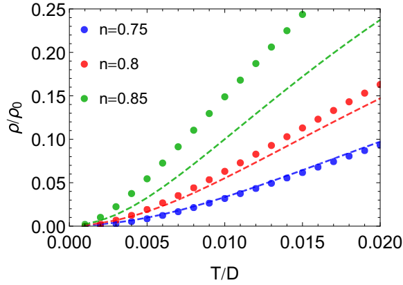
FIG. 2. Comparison of the resistivity computed using the ECFL (symbols) and the DMFT (dashed). \sigma_0 = 1/\rho_0 is the Ioffe-Regel-Mott conductivity. As n gets closer to unity, the ECFL scheme employed systematically underestimates Z relative to the exact DMFT values (see Fig. 6 of Ref. [7]). This lowers the effective Fermi temperature T_{\text{FL}} and simultaneously enhances the magnitude of \rho for T > T_{\text{FL}} , a feature that is prominently visible above. It should be possible to improve the quantitative agreement between the two theories in the future [28].
