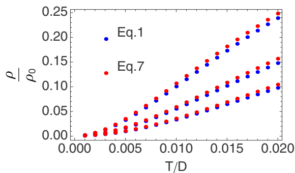
FIG. 4. The exact resistivity [Eq. (1)] compared with the approximation Eq. (7), using the DMFT calculation for n = 0.75, 0.8, 0.85 (bottom to top). Equation (7) is an excellent approximation at all densities for all temperatures. [See Fig. 3(a) for the corresponding figure in ECFL.]
