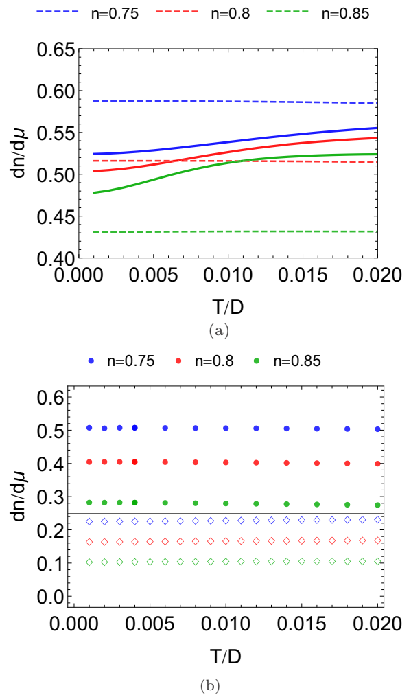
FIG. 8. The charge susceptibilities \chi_c = dn/d\mu , which are related to compressibility \kappa as \chi_c = n^2 \kappa . The numerically exact values versus bubble estimates [Eq. (12)] in panel (a) DMFT (full and dashed lines) and in panel (b) from ECFL (empty diamonds and solid circles).
