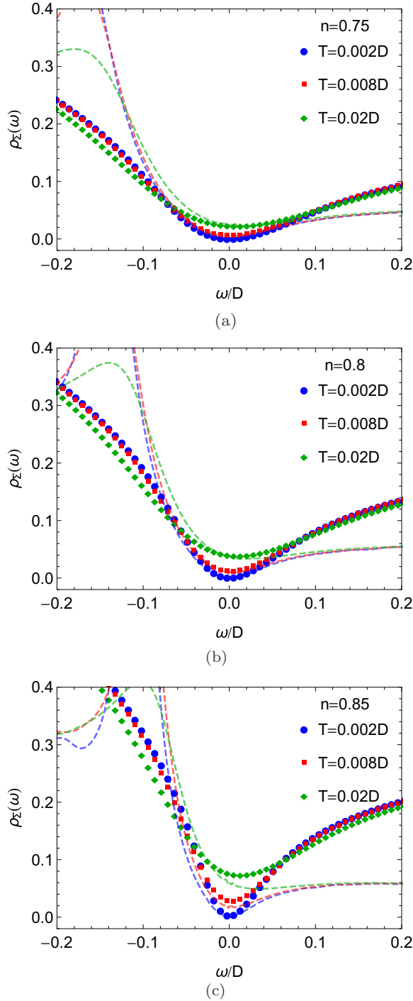
FIG. 9. Single particle decay rates, i.e., the spectral functions of self-energy [ \rho_{\Sigma}(\omega) = -\pi^{-1} \Im m \Sigma(\omega) ] of ECFL (symbols) and DMFT (dashed lines) for a range of temperatures.
