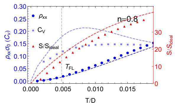
FIG. 13. Resistivity (blue circle), specific heat (light blue square), and entropy (red triangle) as percentage of the ideal entropy at infinite temperature S_{ideal} . The (Schottky) peak in the heat capacity is close to T_{FL} , the onset point of the linear- T resistivity, or the end of the crossover region.
