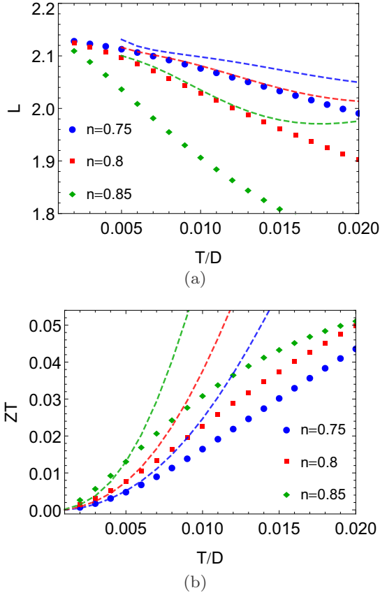
FIG. 16. (a) Lorenz number of ECFL (symbols) and DMFT (dashed lines). The Lorenz number saturates to a constant ( \simeq 2.1 ) which is typically expected for a Fermi liquid at low temperatures. (b) Figure of merit for ECFL (symbols) and DMFT (dashed lines). The low values of ZT found here are typical of normal metals.
