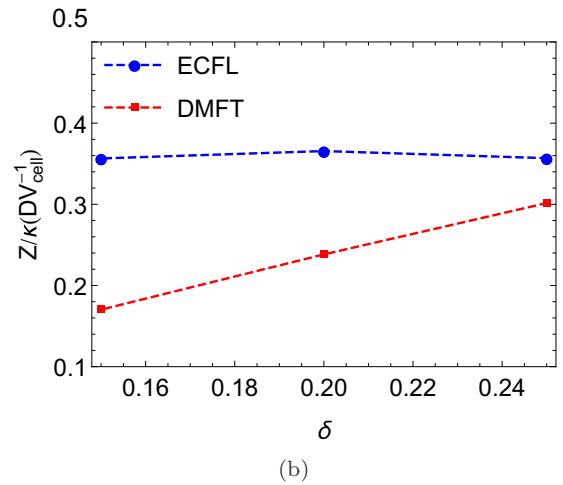
FIG. 6. (a) Compressibility \kappa = n^{-2} \partial n / \partial \mu of ECFL (symbols), DMFT (dashed lines), and free fermions (dotted lines). The DMFT results give a systematically higher value of compressibility than the ECFL theory. (b) Z/\kappa for the lowest temperature T = 0.001D at the three densities considered for ECFL (blue) and DMFT (red). The ECFL result for the compressibility is proportional to the quasiparticle weight Z , unlike the DMFT result which displays some variation. The difference in compressibility between the two theories seems related to the density dependent shift in chemical potentials noted in Fig. 5.
