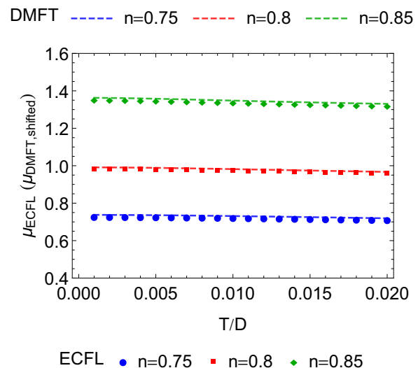
FIG. 5. Chemical potentials at n = 0.75, 0.8, 0.85 for ECFL (symbols) and DMFT (dashed lines). The DMFT results are shifted by a density-dependent constant. After the shift, the chemical potentials almost coincide.
