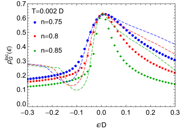
FIG. 10. Local density of states \rho_G^{\text{loc}}(\epsilon) of ECFL (symbols) and DMFT (dashed lines) at T = 0.002D .
