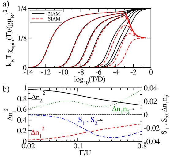
FIG. 5. (Color online) (a) Spin susceptibility for 2IAM (full lines). We choose U_1 = -U_2 = U and \Gamma_1 = \Gamma_2 = \Gamma . For comparison we plot results of the SIAM with the same \Gamma and U (dashed lines). Parameters are U/D = 0.01 and \Gamma/U = 0.02, 0.03, 0.04, 0.05, 0.1, 0.2 , and 0.5 (left to right). (b) Charge fluctuations and correlations in 2IAM for increasing hybridization strength \Gamma .
