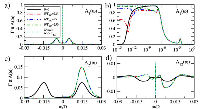
FIG. 9. (Color online) Diagonal ( A_1, A_2 ) and out-of-diagonal spectral densities ( A_{12} ) of the two impurity Anderson model. Same parameters as in Fig. 7.
