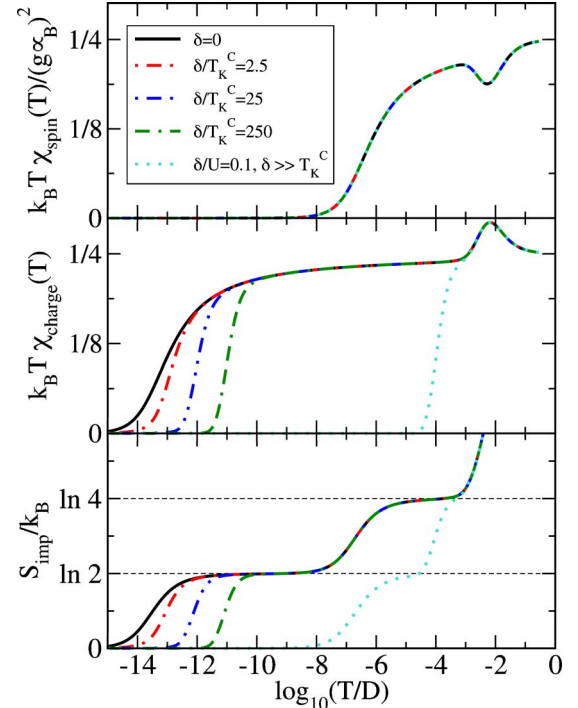
FIG. 7. (Color online) Impurity susceptibilities and entropy for the two-impurity Anderson model. Impurity 1 has U_1=U=0.01 , \Gamma/U=0.05 . Impurity 2 has U_2=-3U=-0.03 and equal hybridization \Gamma . T_K^S/D\sim 1.1\times 10^{-6} , T_K^C/D\sim 2.9\times 10^{-13} . Note that the magnetic susceptibility curves nearly overlap for all values of \delta .
