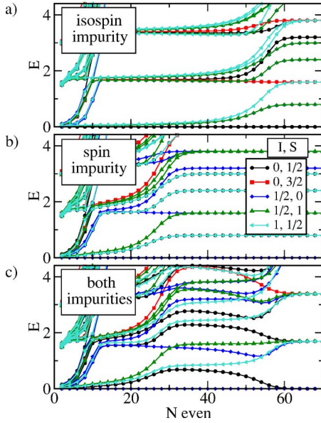
FIG. 6. (Color online) Numerical renormalization group eigenvalue flows for the case when (a) isospin impurity only, (b) spin impurity only, (c) both impurities are present. U_1=U=0.01 , \Gamma_{1,2}/U=0.05 [unless turned to zero in (a) and (b)], U_2=-3U . The levels are labeled by the total isospin and spin quantum numbers (I, S) .
