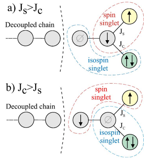
FIG. 4. (Color online) Schematic representation of the strong coupling fixed point Hamiltonian of the spin-charge Kondo model for (a) J_S > J_C and (b) J_C > J_S . For J_C = J_S , the fixed point corresponds to the symmetric combination of (a) and (b).
