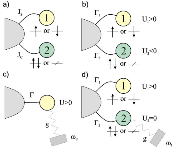
FIG. 1. (Color online) Schematic representations of models discussed in the paper. (a) Spin-charge Kondo model. (b) Two-impurity Anderson model with positive and negative electron-electron interaction. (c) Single-impurity Anderson-Holstein model. (d) Two-impurity Anderson-Holstein model with electron repulsion in one orbital and electron-phonon coupling in the other.
