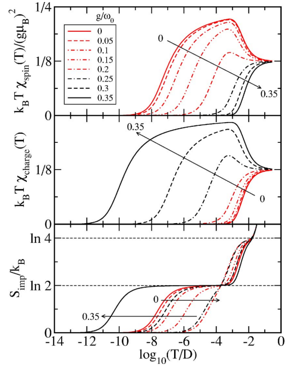
FIG. 10. (Color online) Impurity susceptibilities and entropy for the single-impurity Anderson-Holstein model for increasing e - ph interaction strength g . U/D=0.01 , \Gamma/U=0.04 , \omega_0/D=0.1 .
