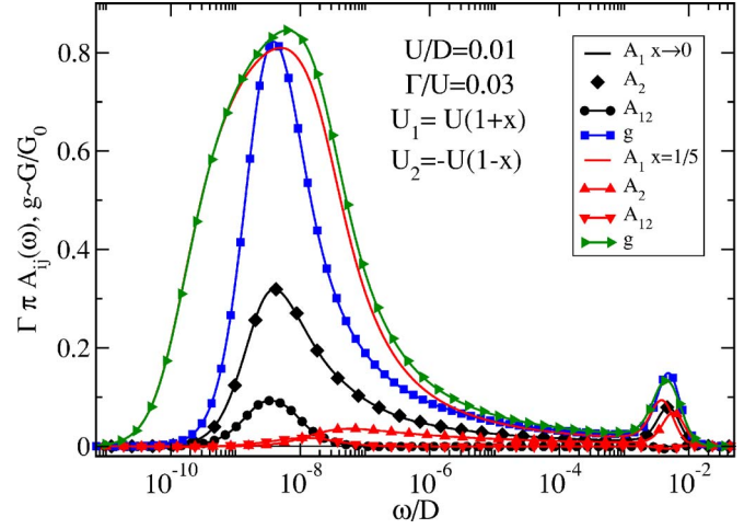
FIG. 8. (Color online) Diagonal ( A_1, A_2 ) and out-of-diagonal spectral density ( A_{12} ) of the two impurity Anderson model for different asymmetry parameters x . We plot only the positive frequencies. Due to the particle-hole symmetry, we have A_i(\omega) = A_i(-\omega) and A_{12}(\omega) = -A_{21}(-\omega) .
