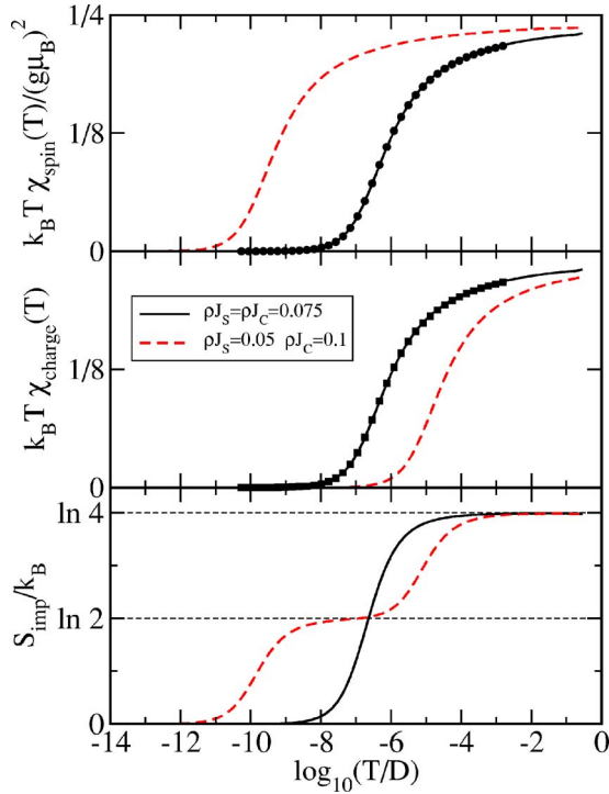
FIG. 2. (Color online) Impurity susceptibilities and entropy for the spin-charge Kondo model. Filled symbols are a fit to the exact Bethe-ansatz results for susceptibility. From this fit we deduce T_K^S = T_K^C = 2.7 \times 10^{-7} D , in approximate agreement with T_K = D \sqrt{\rho J} \exp(-1/\rho J) = 4.4 \times 10^{-7} D .
