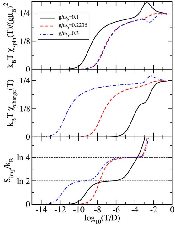
FIG. 11. (Color online) Impurity susceptibilities and entropy for the two-impurity model with one Holstein impurity with \omega_0/D = 0.1 and varying e -ph interaction strength g , and one Anderson impurity with U/D = 0.01 . Both impurities are coupled with \Gamma/D = 0.0004 to the conduction band.
