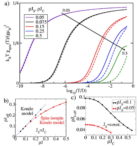
FIG. 3. (Color online) (a) Spin susceptibilities in the SKCM model with J_C = J_S (solid lines) compared with spin susceptibilities in the corresponding SKM with the same Kondo exchange constant J_S (dashed lines). (b) Effective exchange constant J_{\text{eff}} as a function of J_S for the case J_C = J_S (red, circles), compared with the single-impurity results (black, squares). Blue straight line is a fit to the single-impurity results and serves as a guide to the eye. (c) Effective exchange constant J_{\text{eff}} as a function of the charge Kondo exchange constant J_C while keeping the bare spin exchange constant J_S constant at \rho J_S = 0.1 (black, circles) or \rho J_S = 0.05 (red, squares).
